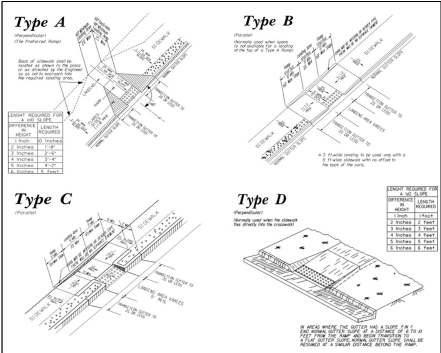
Figure 4-11C – CONCRETE SIDEWALK WHEELCHAIR RAMPS TYPES
