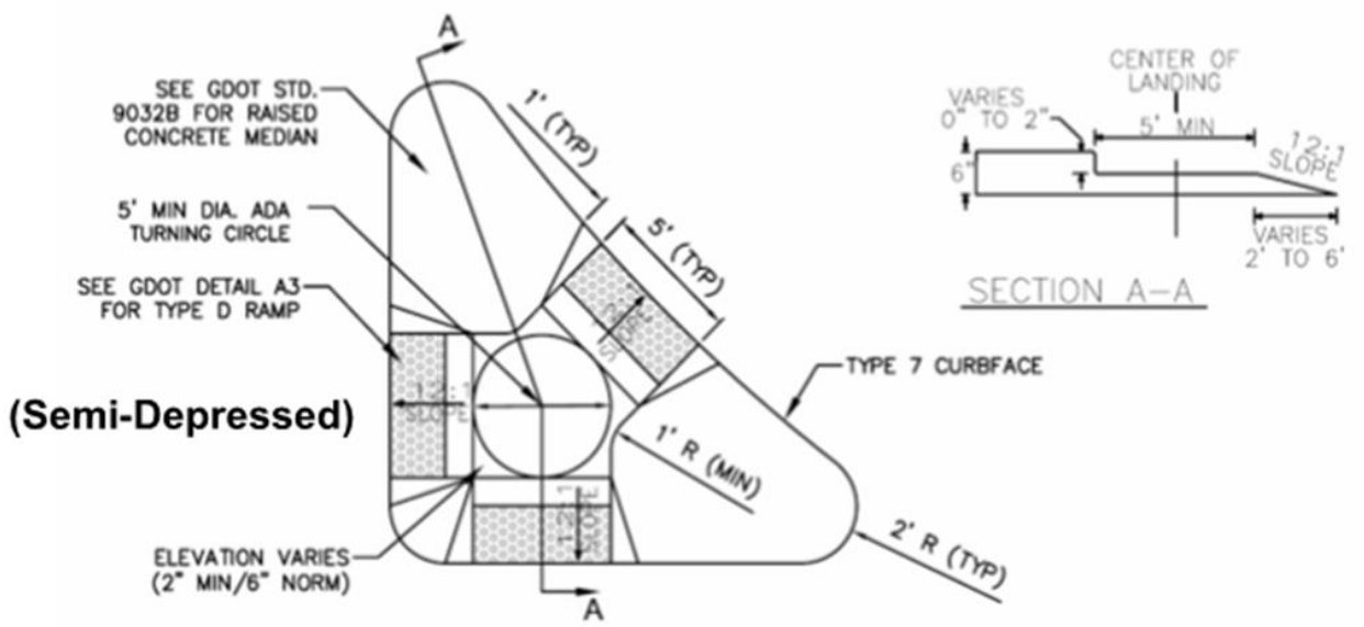
Figure 4-9B Raised Island Detail
